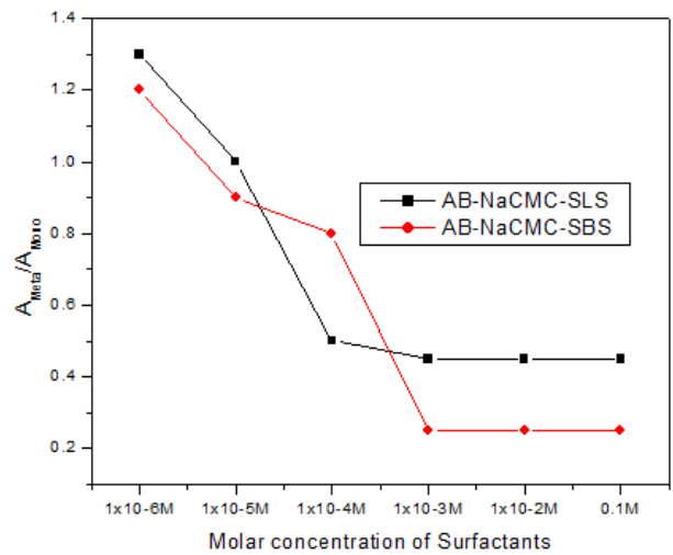
Figure 9. Reversal of metachromasy on addition of surfactants (AB-NaCMC)
